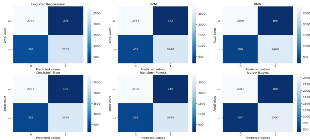
Figure 1. Confusion matrix of results of application traditional machine learning algorithms
